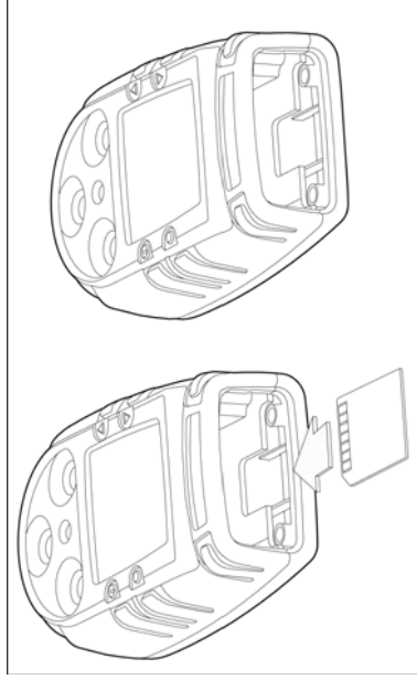
Figure 5. Inserting the MultiMediaCard (MMC)
