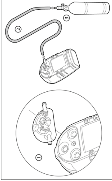
Figure 4. Attaching the Gas Cylinder to the Detector
